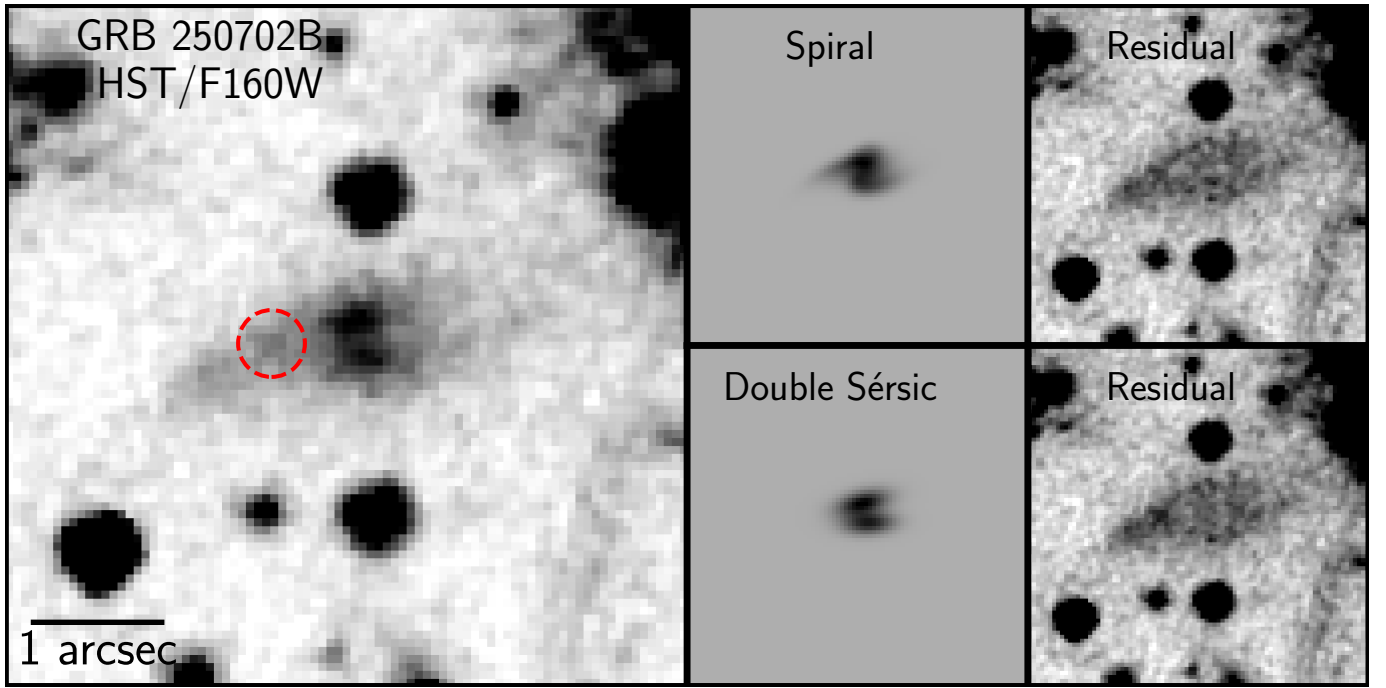
Figure 5. Left panel: HST image of the host galaxy of GRB 250702B in the F160W filter. The location of the transient is marked by a red circle. Top middle panel: GALFIT model of best-fitting single Sérsic light profile and power-law spiral arms. Top right panel: the residual image of GALFIT after subtracting the spiral plus Sérsic model. Bottom middle panel: GALFIT model of best-fitting double-Sérsic light profiles. Bottom right panel: the residual image of GALFIT after subtracting the double-Sérsic model. In all images north is up and east is to the left.
