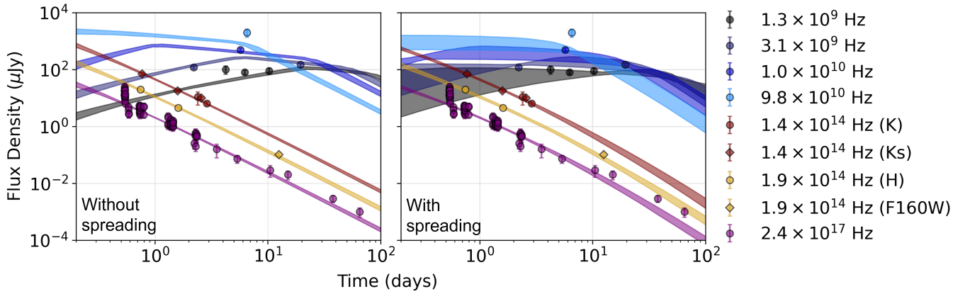
Figure 3. Radio, X-ray, and infrared detections of the counterparts to GRB 250702B. The 1\sigma posteriors from VegasAfterglow fit to these data are shown as shaded regions. The left panel shows the fitting results without jet spreading enabled, and the right panel shows the results with jet spreading enabled.
