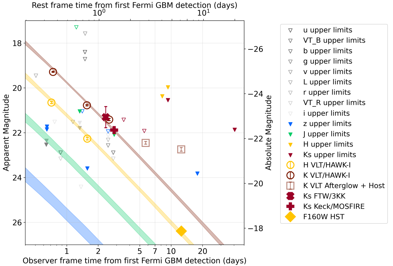
Figure 2. Light curve of the observed infrared counterpart of GRB 250702B, including UV and optical upper limits. t = 0 is defined as the time from 2025 July 2 13:09:02 in the observer frame. Rest-frame time from the first Fermi trigger and absolute magnitudes are calculated at z = 1.036 (B. P. Gompertz et al. 2025) without additional K -correction and are corrected for Milky Way extinction using the dust maps by E. F. Schlafly & D. P. Finkbeiner (2011). Error bars represent 1\sigma confidence, and upper limits represent 5\sigma confidence. UV/optical observations are denoted in gray scale, with lighter colors representing longer wavelengths; NIR observations are colored blue to red according to their wavelengths. Data presented for the first time in this work, together with our host-model-subtracted photometry of the HST data first published in A. J. Levan et al. (2025), are represented by filled symbols, whereas data from the literature are represented by open symbols (see Table 1). Later VLT epochs with likely host contamination are denoted separately as squares and were excluded from modeling. For z , J , H , and K bands, the 1\sigma region in the posteriors for the best-fit forward shock model described in Section 3.1 is shown as a shaded region.
