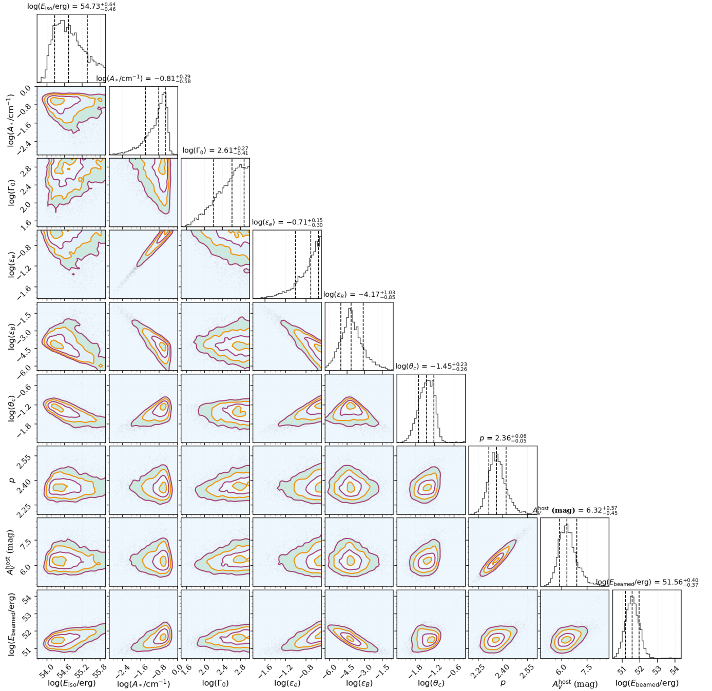
Figure C3. Posterior distributions of the jet parameters derived using VegasAfterglow to fit the available multiwavelength with a nonspreading top-hat jet constrained such that \Gamma_0\theta_c > 1 .
