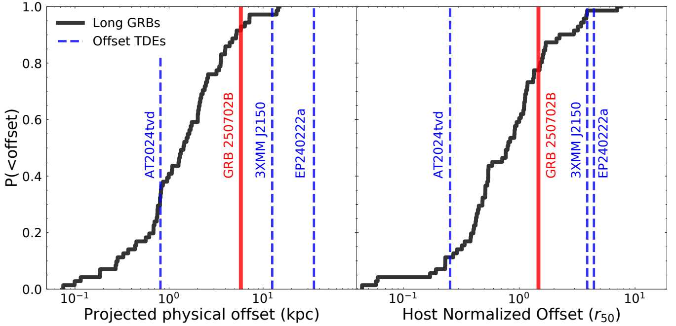
Figure 6. Left: the projected galactocentric offset of GRB 250702B compared to offset TDEs (Y. Yao et al. 2025) and the cumulative distribution for long GRBs (P. K. Blanchard et al. 2016). Right: same as the left panel, but for the host-normalized offset ( r/r_{50} ). The offset TDE candidates 3XMM J2150 (D. Lin et al. 2018, 2020), EP 240222a (C. C. Jin et al. 2025), and AT 2024tvd (Y. Yao et al. 2025) are believed to be associated with an IMBH.
