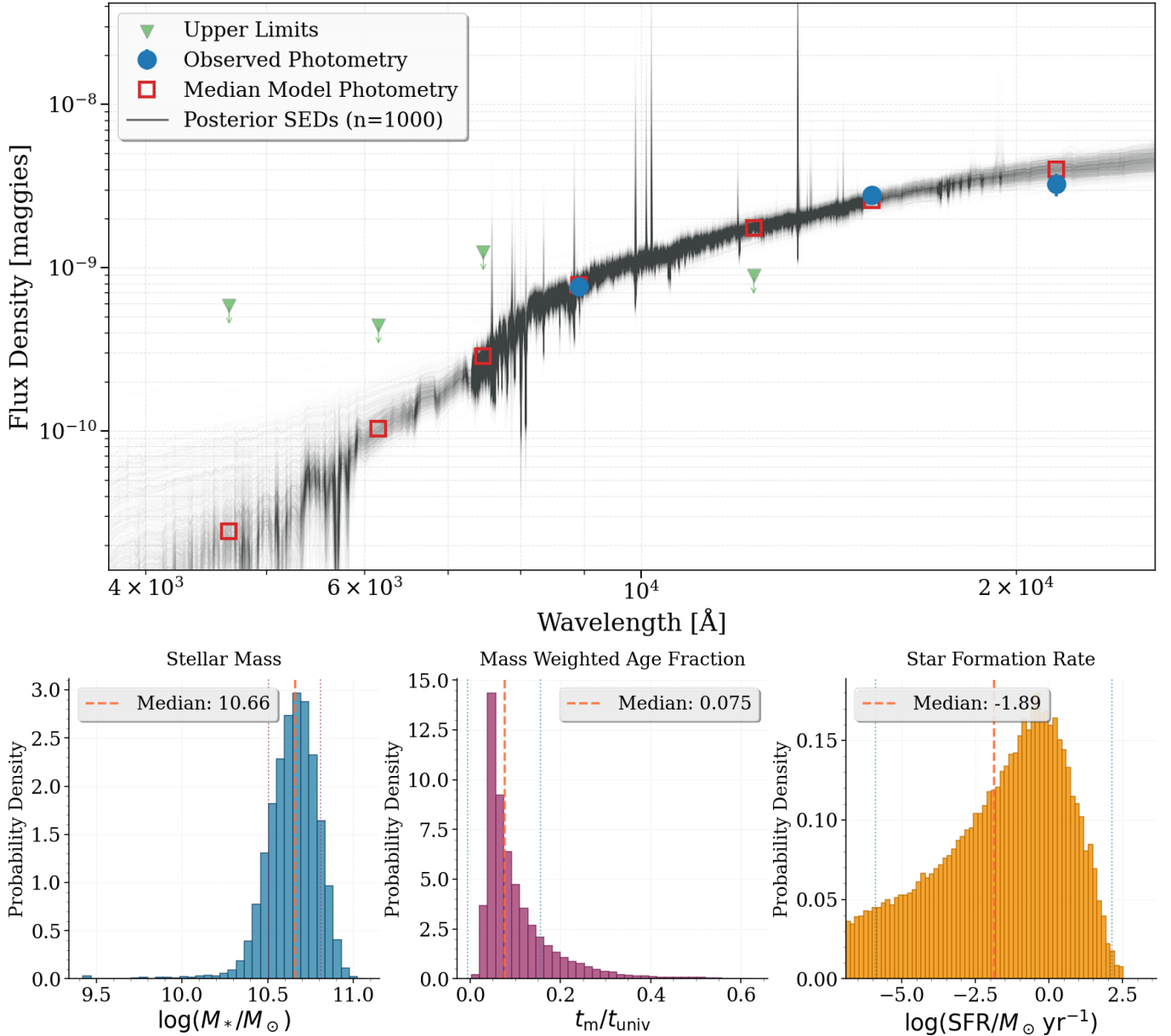
Figure 4. Top panel: observed host photometry ( z , F160W, K_s with g and r upper limits) overlaid with 1000 randomly drawn galaxy SEDs from the prospector posterior distributions (Figure C4). The data are corrected for Milky Way extinction prior to modeling. Bottom left: posterior distribution of stellar mass from prospector modeling. Bottom middle: posterior distribution of mass-weighted age from prospector modeling. Here we show it in units of 5.71 Gyr (the age of the Universe at z = 1.036 ). Bottom right: posterior distribution for SFR from prospector modeling.
