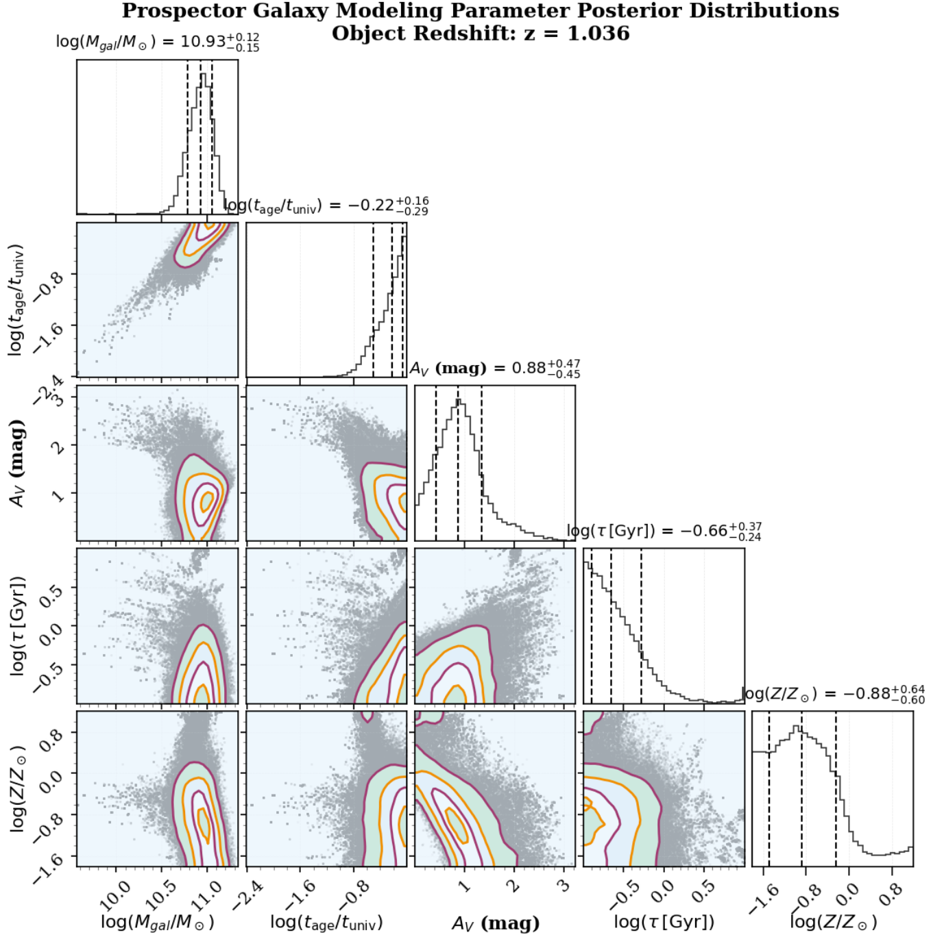
Figure C4. Posterior distributions of our host galaxy SED fitting results using prospector . We note that M_{\text{gal}} refers to the total mass formed and not the galaxy's stellar mass. See also Figure 4.
